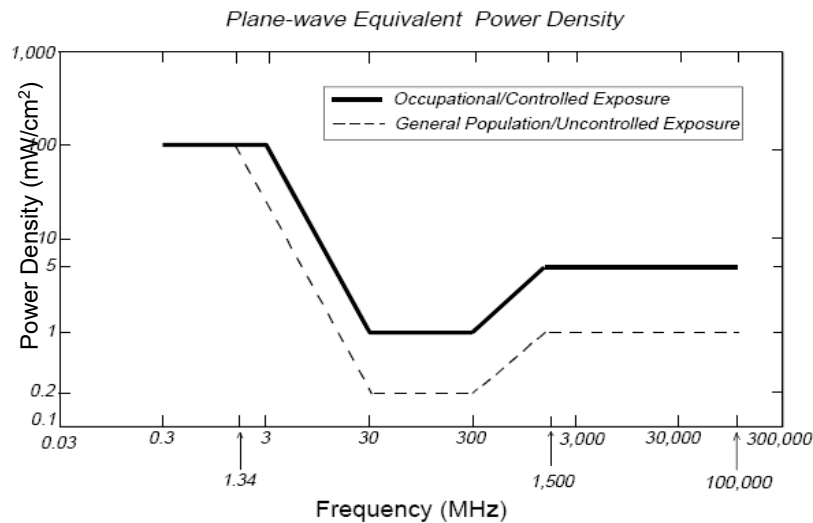
Figure 1. FCC Limits for Maximum Permissible Exposure (MPE)
